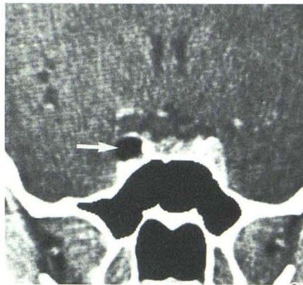
Fig. 4.—Direct coronal CT shows low-attenuation lesion (arrow) within right cavernous sinus in 24-year-old man with 3-week history of complete third nerve palsy and retroorbital throbbing headache. Working diagnosis of epidermoid tumor lacked surgical proof.
