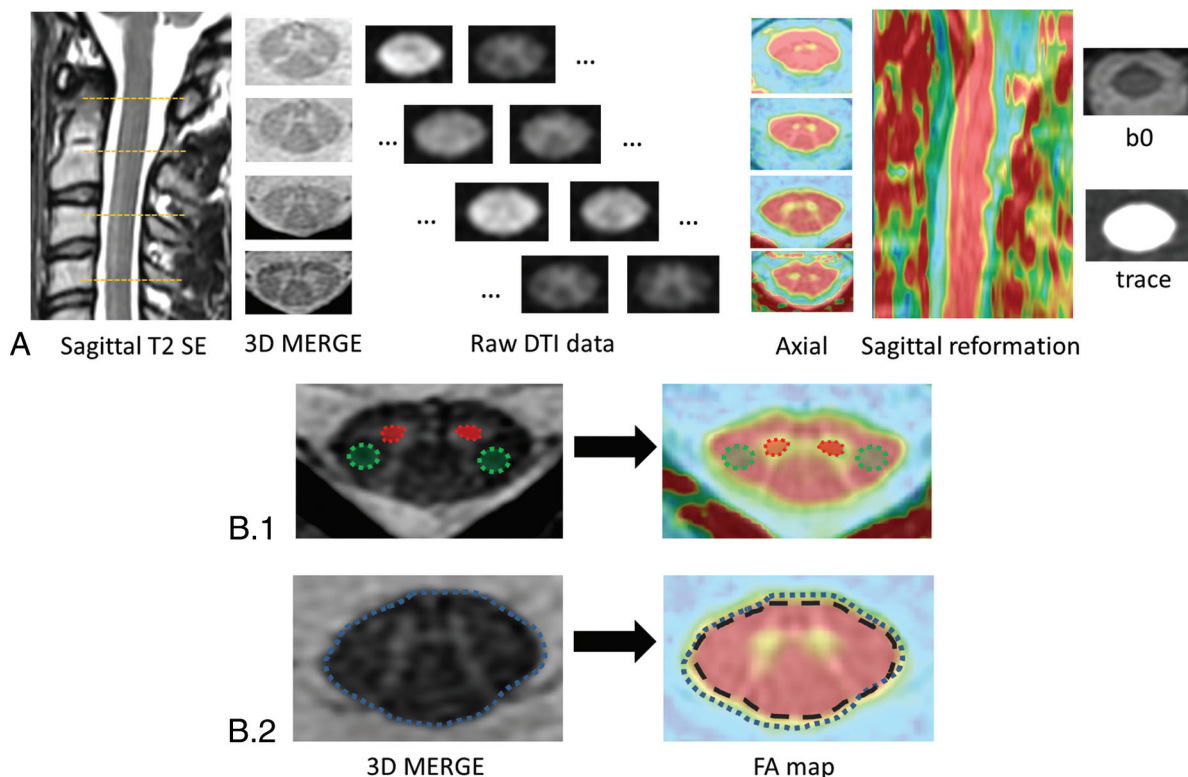
FIG 1. Postprocessing pipeline and analyses. A, Four sections were analyzed in detail: C1, C2, C3, and C4. Raw data diffusion-weighted images were treated for eddy current correction before generation of DTI parameters. We focused on FA because this parameter is the most commonly used. Fusions of FA and 3D-MERGE were created at these 4 levels as well as reconstructed on the sagittal orientation to facilitate the identification of distortions and pixel misregistration. B, ROI positioning: ROIs (B1) were manually delineated on 3D-MERGE, on the right and left anterior horns of the cord (red area) for gray matter, and on the right and left corticospinal tract (green area) for white matter, and then propagated on the coregistered FA map. B2, If needed, ROIs were manually adjusted to account for FA map distortion. Furthermore, because of the partial volume effect at the interface between CSF and the FA map, ROIs of the full section (blue dotted line, whose surface corresponded to S_{[Full\ Section - Merge]} ) were adjusted to remove the pixels subject to artifacts at the periphery of the ROI (black dashed line, whose area corresponded to S_{[Full\ Section - FA]} ).
