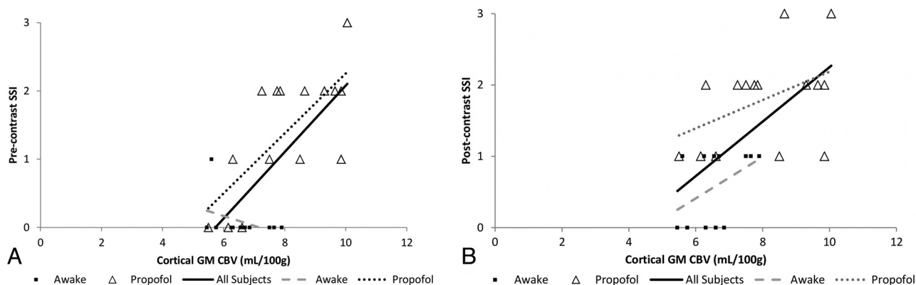
FIG 2. Relationship of CBV with pre-contrast (A) and post-contrast (B) FLAIR SSI. Significant correlations ( P < .05 ) are in black.
