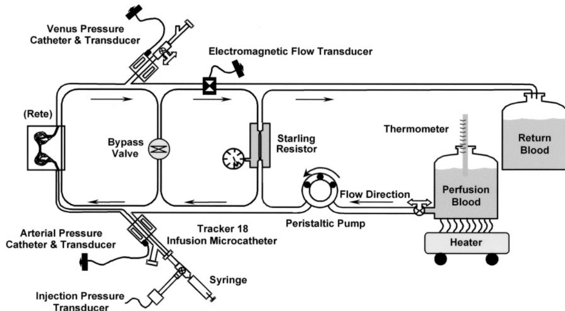
FIG 1. Illustration of the perfusion apparatus used in the chronic swine AVM model.
