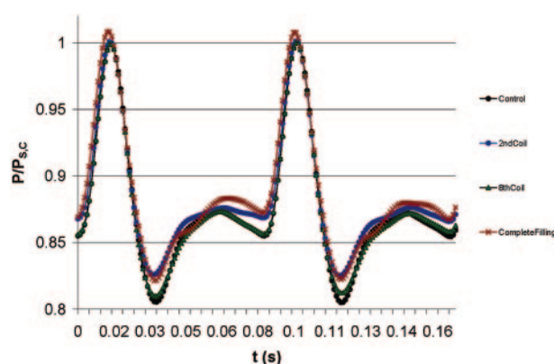
FIG 1. Intraaneurysmal pressure measurements of the non-treated aneurysm model (control), after placing two structural coils (2nd coil), after placing six hydrogel-coated coils (8th coil), and for the complete filling (14th coil). Measurements were normalized with the measured pressure at peak systole for the control case, P_{sc} . The slight difference between the curves remains within the measurement error ( \pm 2 mmHg).
