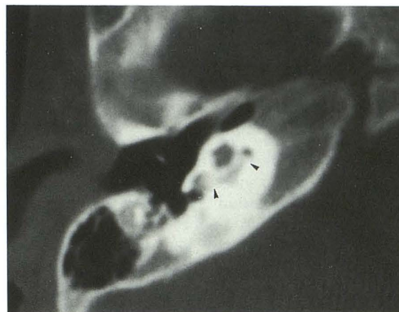
Fig. 7. Cochlear ossification in a child with difficult electrode placement during cochlear implantation (Johnson et al). An axial CT section through the right cochlea shows several focal ossifications within the cochlear lumen (arrowheads).
