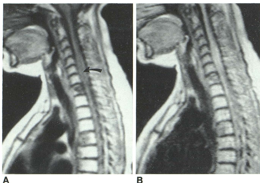
Fig. 4.—Intramedullary metastasis from lung carcinoma. A, SE 500/30. Lower cervical cord is enlarged; central part appears to contain cavity (arrow). Loss of normal marrow signal from T1 and T5 vertebral bodies represents bone metastases. B, SE 1000/60. Increase in signal from lesion. Other findings essentially unchanged.
