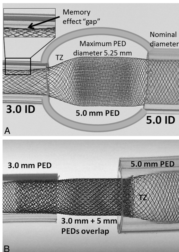
FIG 2. Consequences of device oversizing and the proposed solution. A , A model of a fusiform aneurysm with 3.0- and 5.0-mm landing zones, bridged by a single 5 × 20 mm device. A transition zone (TZ) of minimum coverage is created as the device is constrained from its fully opened state into the 3-mm landing zone. Despite adequate length of the “landing zone” at the 3.0-mm end, the “shape memory” of the transition zone, TZ, nevertheless produces a “gap” where the device remains unapposed to the inner wall of the tube. B , To address these issues, 2 devices are required, each of which is appropriately sized for its recipient artery. The first 3.0-mm device is deployed from the 3.0-mm-diameter vessel into the 5-mm recipient vessel, following which a second 5.0-mm diameter device is telescoped into the first, with the 5.0-mm device anchored into its 5.0-mm vessel. Thus, the transition zone, TZ, is shifted outside the aneurysm, while the aneurysmal segment receives the benefit of double-coverage.
