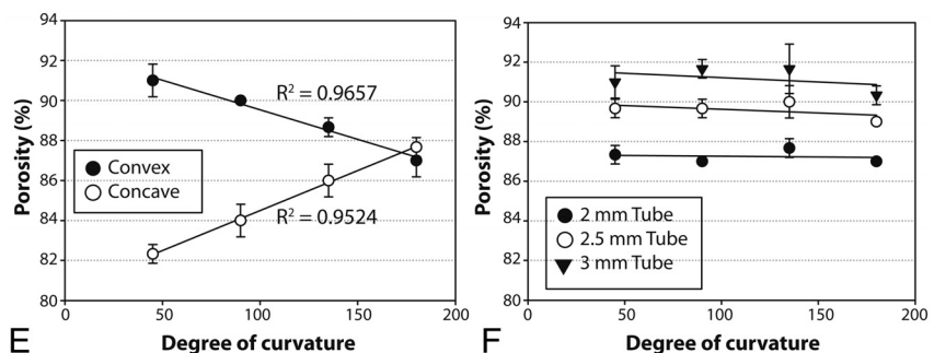
FIG 5. Concavity at 45° (A, C) and convexity at 135° (B, D) of expansion Zone 3 before (A, B), or after (C, D) the stent is compacted. Curvatures affect the porosity of the convexity and concavity sides of the compaction Zone 3 (E), whereas the transition Zone 2 remains virtually unchanged by comparison (F, showing the porosity of the transition Zone 2 with different tubes and different curvatures).
