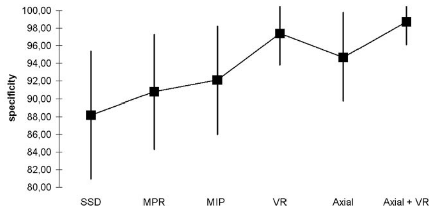
Fig 5. Graph shows the specificity of SSD, MPR, MIP, VR, axial, and axial + VR. Mean values (■) and 95% confidence intervals (error bars) are indicated
