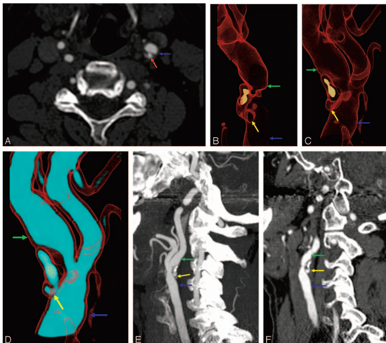
Fig 3. A 78-year-old man with TIA. Ulcerated plaque of the left CCA. Axial scan (A) shows ulcerations in a calcified plaque; the atheromatous plaque involved the common carotid artery, the carotid bifurcation, and internal carotid artery origin. This ulcer is proximal to the point of maximum stenosis (90% NASCET). The ulceration was easily detected using VR technique with 1 histogram (B) and 2 histograms (C, D). Ulceration was less clearly visible using MIP and MPR reconstruction (E, F). Note: B is an internal visual, where the lumen is cut to clarify the ulcers. (red arrow in axial image and yellow arrows in VR, MIP, and MPR images, ulceration; green arrows, ICA; blue arrows, CCA)
